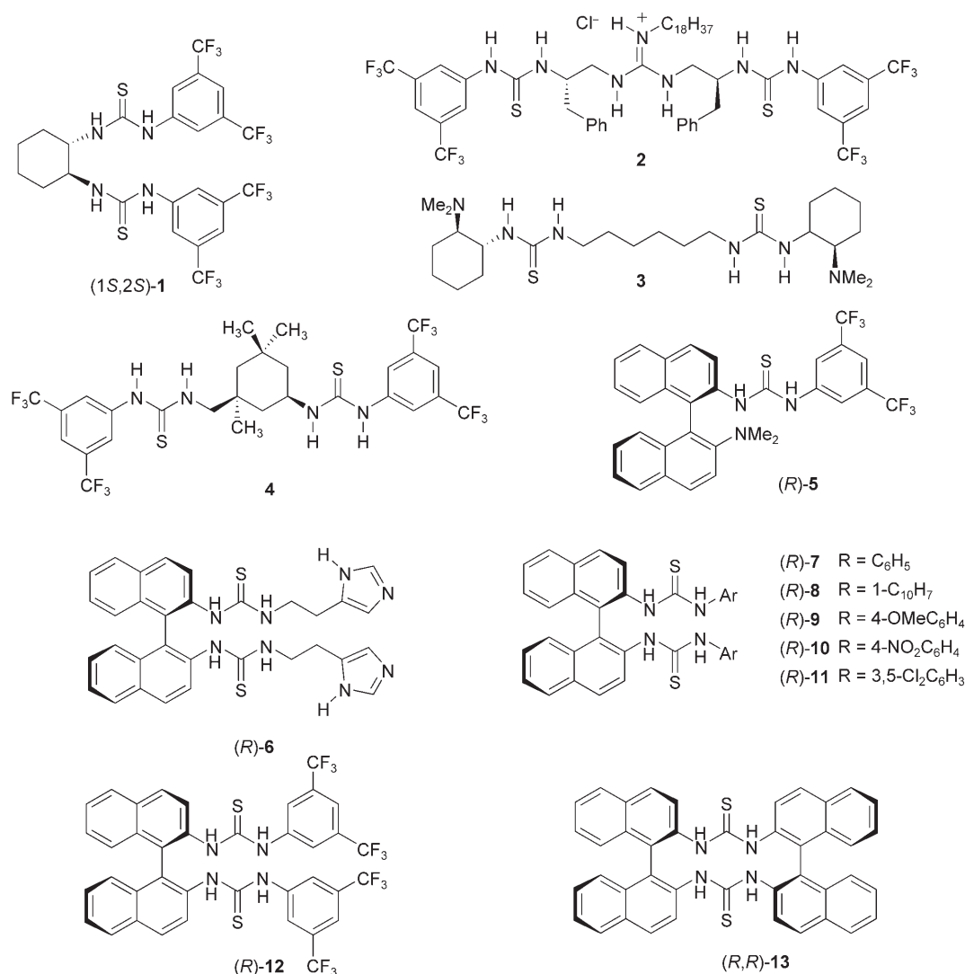
Figure 1. Chiral thioureas and bis-thiourea organocatalysts.
